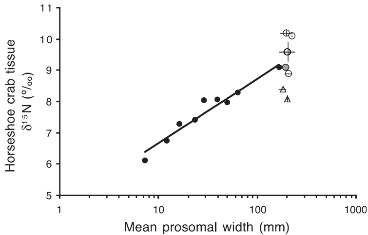
Fig. 6. Change in \delta^{15}\text{N} signatures of horseshoe crabs with increasing prosomal width. Data points correspond to juveniles \sim 7 –168 mm in size (●) and adults (●) collected at Nauset Beach, and adults collected from 7 other locations in the Pleasant Bay system (open symbols), separated to show where crabs foraged (○) and where foraging did not occur (△). Error bars show standard error. Model II regression yielded a best-fit line to the Nauset Beach juvenile data, y = 0.89\ln(x) + 4.62 , R^2 = 0.95 , F_{\text{reg}} = 162.08 , P < 0.001 .
