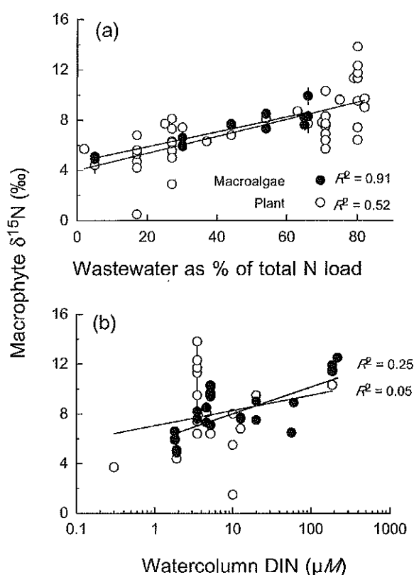
Fig. 3. (a) Wastewater as a percentage of total N load as calculated with the N-loading model of Valiela et al. (1997, 2000) vs. \delta^{15}\text{N} of macrophytes used in this study divided into groupings of macroalgae and plants. (b) Mean annual water-column dissolved inorganic nitrogen (DIN) concentrations vs. \delta^{15}\text{N} of macrophytes used in study divided into groupings of macroalgae and plants.
