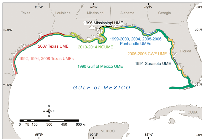
Fig. 1. Historical Gulf of Mexico mortality events (1990–2009) and the northern Gulf of Mexico unusual mortality event (NGUME). The geographic extent of each event is color coded to match the event title. CWF: central west Florida
