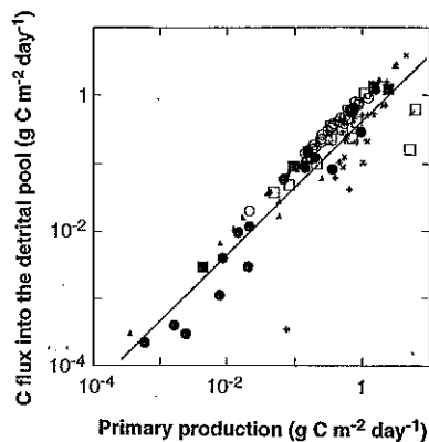
Fig. 1. The relation between C flux into the detrital pool and primary production (both in units of grams of C per square meter per day). The solid line depicts the regression equation fitted to the data. Symbols represent (*) plankton, (●) benthic microalgae, (Δ) macroalgal beds, (▲) freshwater macrophyte meadows, (■) seagrass meadows, (□) grasslands, and (○) forests.
